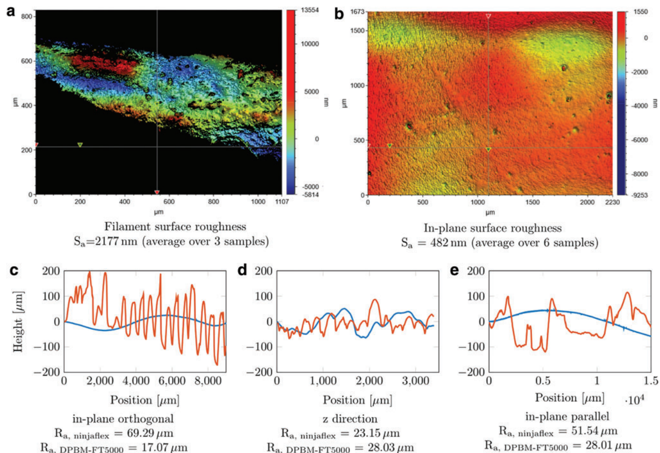
FIG. 8. (a, b) Surface roughness measured by white light interferometry, no value was obtained in the black areas of (a) due to the cylindrical shape of the filament. (c–e) Roughness profiles in different directions of unidirectional printed samples DPBM-FT5000 (blue) and NinjaFlex (red). Both samples printed on a LulzBot TAZ 6 with a layer height of 0.3 mm and nozzle size 0.5 mm. NinjaFlex printed at 230°C. Profiles measured with a stylus radius of 2.5 \mu\text{m} and force of 3 mg, tilt of the sample is accounted for. Color images are available online.
