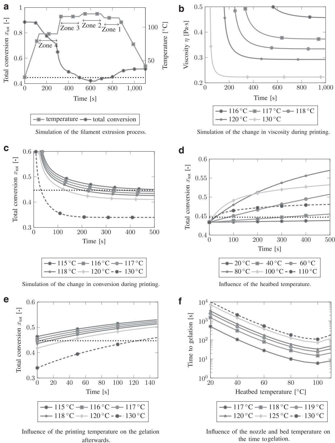
FIG. 6. (a) Simulations (steps of 1 s) of the extrusion process show that the material only degels (total conversion below the (de-)gelation line of x_{gel} = 0.447 ) for \sim 300 s. Screw rotation speed is set at 2 rpm. (b) Simulations of the change in viscosity during printing at various temperatures show that at a lower print temperature, the kinetics of degelation are slower and the material will remain more viscous. (c) At higher temperatures, degelation can take place faster. (d) The heated bed temperature has a large influence on the time it takes for the printed material to gel. This time should be minimal to allow faster printing and prevent flow of the printed material. Consequently a higher temperature is beneficial, with an optimum at 100°C. (e) A higher printing temperature has a negative effect on the time to gelation on the heatedbed. (f) The time to gelation depends on the print temperature and the heatedbed temperature (lines). Gelation happens earlier at low print temperatures and high heatedbed temperatures.
