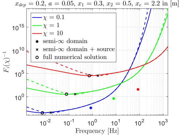
Figure 5. Inverse Fisher information matrix based on (3) assuming a sinusoidal boundary input, a sinusoidal source input, as function of frequency for three different values of \chi . The * give the minima of F_i with respect to frequency as were shown in Fig. 3. The dashed lines with minima \times are the results for F_i^{-1} using approach A) as defined in (3). The full lines with minima \circ give the results for F_i^{-1} using approach B).
