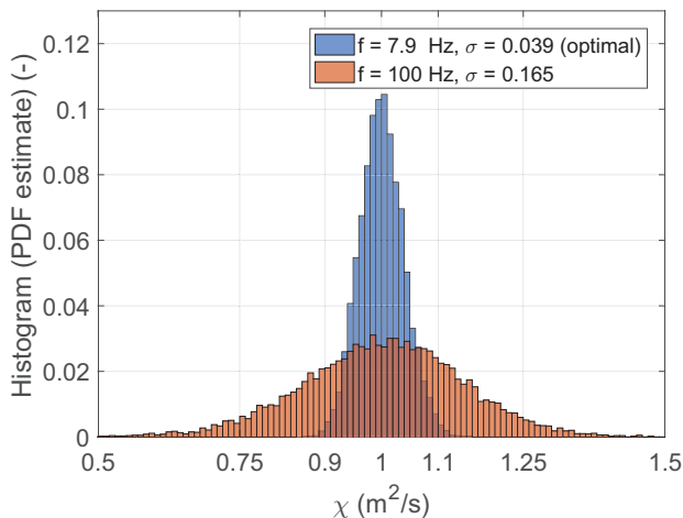
Figure 4. Histograms of 10000 estimations of the diffusion coefficient based on (3) where the optimal modulation frequency is used and a non-optimal frequency is used. Input of the simulation is \chi = 1 and a noise level of \sigma = 0.01 for \Theta(\omega, x_x) used to avoid estimates of \chi around 0. The optimal modulation frequency is invariant for a change in \sigma in the case of only input or output noise.
