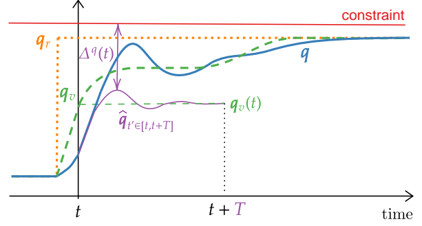
Fig. 3: Trajectory-Based DSM Principle – An arbitrary reference \mathbf{q}_r is given to the trajectory-based ERG, which returns the feasible reference \mathbf{q}_v that can be applied to the system without causing any constraint violations, resulting in the real robot motion \mathbf{q} . Before time t , a step reference is reached by the robot (i.e. \mathbf{q}_r = \mathbf{q}_v = \mathbf{q} ), whereafter another step reference \mathbf{q}_r is given to the system. Starting from the current robot states (\mathbf{q}(t), \dot{\mathbf{q}}(t)) at time t , the trajectory-based DSM predicts the robot dynamics \hat{\mathbf{q}}_{t' \in [t, t+T]} over a finite time horizon T for a constant applied reference \mathbf{q}_v(t) . The minimal distance between the predicted states and the constraint is denoted by \Delta^q(t) and denotes the guaranteed safe rate of change of the applied reference, i.e. \dot{\mathbf{q}}_v . In a similar way constraints on other variables can be accounted for.
