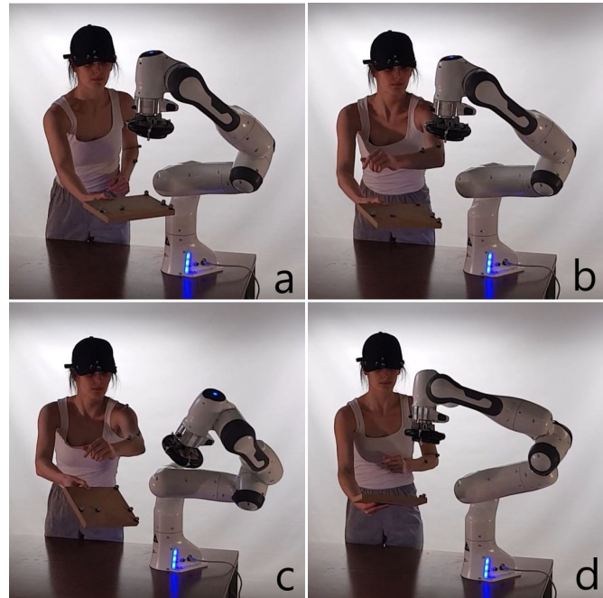
Fig. 1: Experimental Validation of the Trajectory-Based ERG. a) the robot's end-effector pose reference is defined using a wooden plate with reflective markers, b) the arm of the human operator gets in between the robot and its reference, c) the robot safely moves away from the human, d) the robot goes back to its reference once it is safe to do so. See https://youtu.be/UzbhMzcKSbE for the full video.
