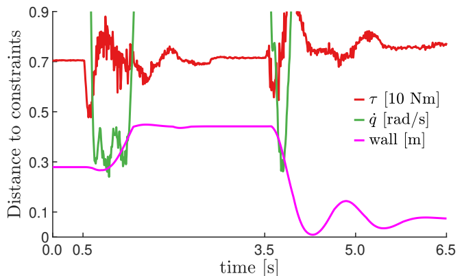
Fig. 9: Static Obstacle Environment With Wall Constraint DSM (Exp 3) – In this experiment \Delta^w is taken into account to compute the overall \Delta . Thus, the applied reference is slowed down enough to avoid any constraint violations.
