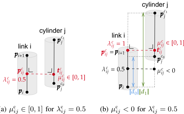
Fig. 16: Parametrization of Robot Link i and Cylinder j – The distance \|\mathbf{p}_{ij}^c \mathbf{t}_{ij}^c\| defines the shortest distance between link i and cylinder j in the case they are parallel to each other.
