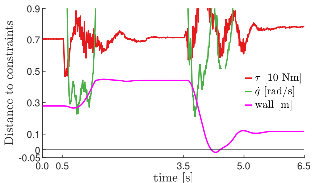
Fig. 7: Static Obstacle Environment without Wall Constraint DSM (Exp 2) – Although \Delta^{\dot{q}} < 0 around 3.6 s in Fig. 6, the distance of the real (not predicted) \dot{q} to its constraints is not violated. However, since \Delta^w is not taken into account, the wall constraint is violated around t = 4.3 s by almost 2 cm.
