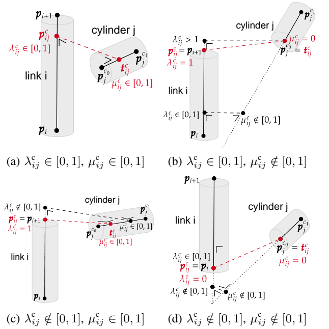
Fig. 17: Parametrization of Robot Link i and Cylinder j – The distance \|\mathbf{p}_{ij}^c \mathbf{t}_{ij}^c\| defines the shortest distance between link i and cylinder j in the case they are skew to each other.
